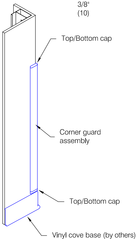
Application Diagram
